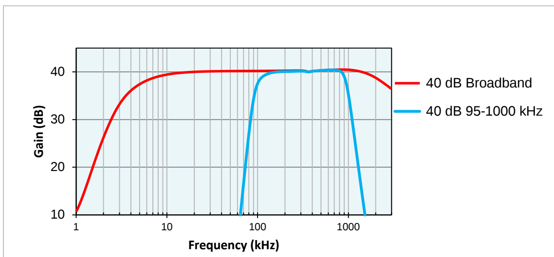
Figure 3: Frequency response of AEP3N with two different band-pass filters. "Broadband" refers to bypass-filter. Other frequency filter available, see table below.
