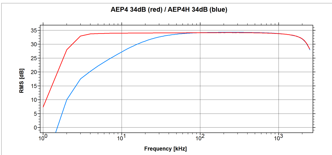
Figure 9: Frequency response of AEP4 and AEP4H preamplifier
