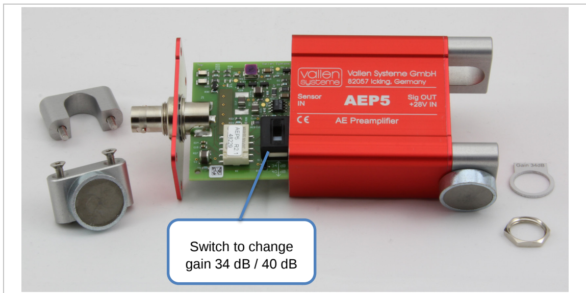
Figure 6: disassembled AEP5 with pulled out PCB assembly for changing gain setting.
