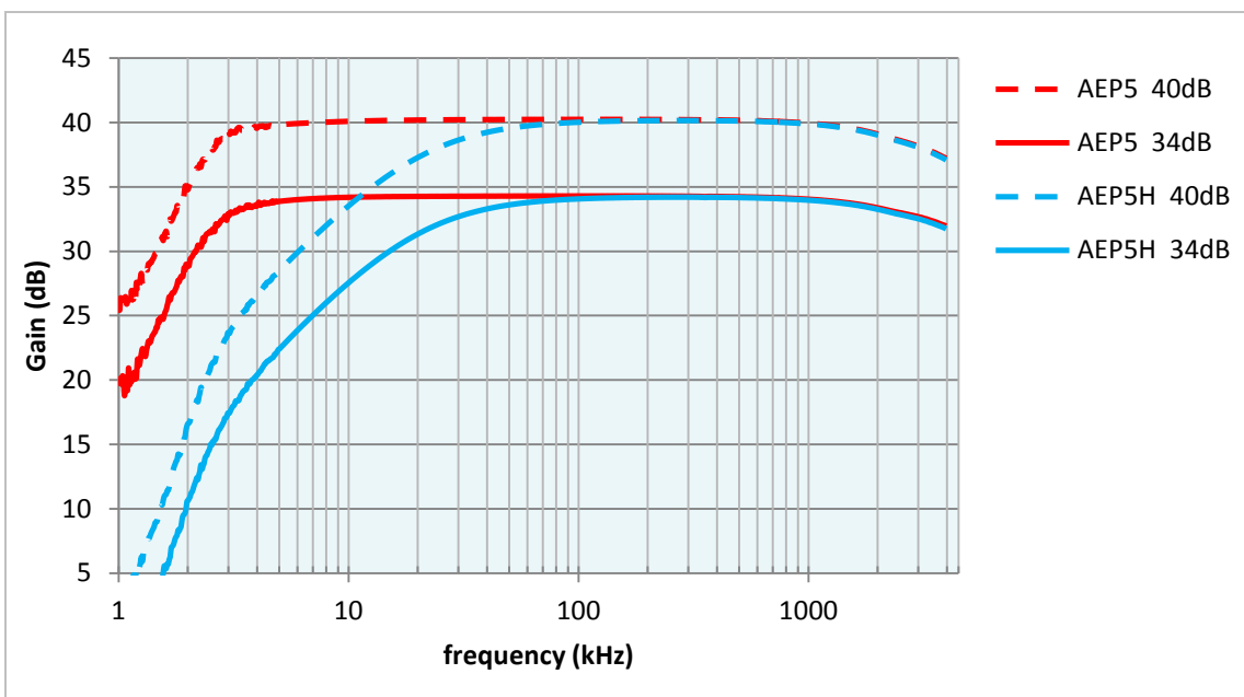
Figure 5: Frequency response of AEP5 and AEP5H preamplifier
